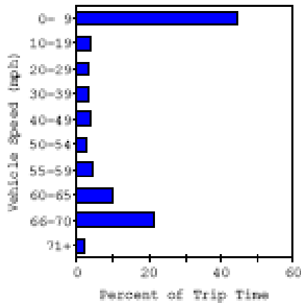
Vehicle Speed Histogram
