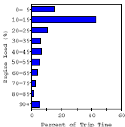
Engine Load Histogram
